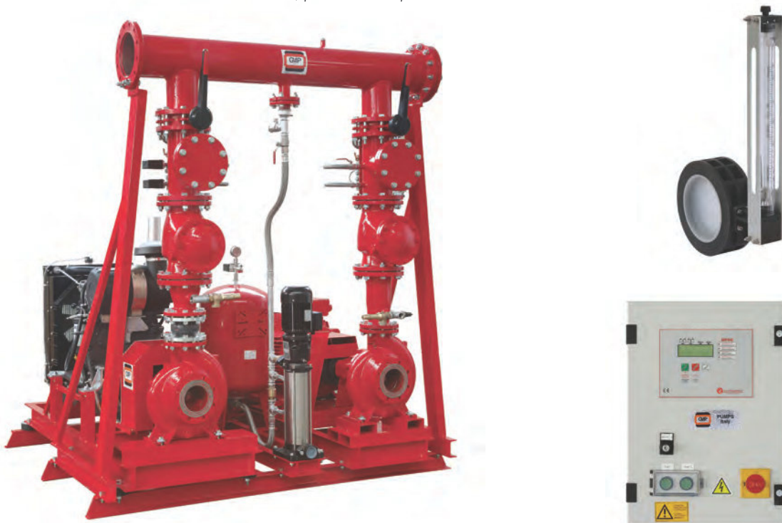
“ Version ED” costituita da 1 elettropompa primaria - 1 motopompa diesel di riserva e - 1 elettropompa jockey “ED version” 1 main electric pump - 1 auxiliary diesel motor pump and - 1 jockey electric pump “Version ED” 1 électropompe primaire - 1 motopompe diesel auxiliaire et - 1 électropompe jockey
